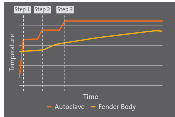
Figure 2: Temperature increase while curing
